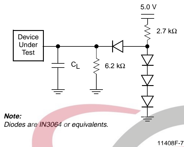
Figure 3. Test Setup
